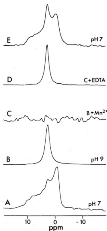
FIGURE 4: 81-MHz ^{31}\text{P} NMR spectra of a single aqueous dispersion of 1-C18:1c-PE at 20^\circ\text{C} : (A) at pH 7; (B) at pH 9; (C) \text{MnCl}_2 was added to (B) to a final concentration of 2 mM; (D) EDTA was added to a final concentration of 5 mM; (E) the pH of the sample was lowered to pH 7.
