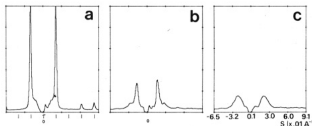
FIGURE 3: Small-angle X-ray scattering (SAXS) intensity (arbitrary units) from a 25% w/w dispersion of 1-C18:1c-PE vs. s = (\sin 2\theta)/\lambda (in units of 0.01 \text{ \AA}^{-1} ) where 2\theta is the scattering angle and \lambda = 1.54 \text{ \AA} is the Cu K \alpha X-ray wavelength. For Figures 3, 10, and 11, the zero angle of scatter (behind the beam stop shadow) is indicated by a zero below the abscissa. Equidistantly spaced tick marks indicate the expected peak positions of a lamellar lattice, and nonequidistantly spaced tick marks are for a hexagonal lattice. (a) -9^\circ\text{C} , lamellar basis = 47.6 Å; (b) 1^\circ\text{C} , largest peak corresponds to 58 Å; (c) 11^\circ\text{C} , peaks correspond to approximately 45 Å. Exposure times were 300 s.
