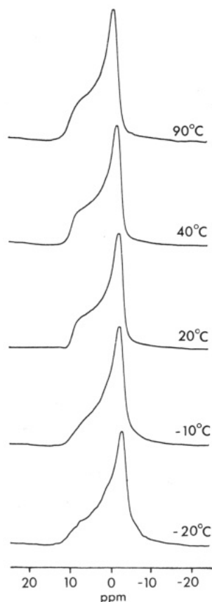
FIGURE 1: 81-MHz ^{31}\text{P} NMR spectra of aqueous dispersions of 1-C18:1c-PE at pH 7 between -20 and 90^\circ\text{C} .
