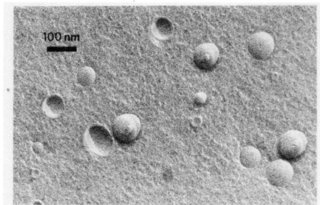
FIGURE 8: Freeze-fracture electron microscopy of a di-C18:1 c -PC/1-C18:1 c -PE (1:1) mixture dispersed at pH 7 and then raised in pH to 10.4 and back to 7.
