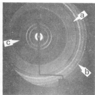
FIGURE 2: Diffraction pattern from a roughly 20% (w/w) dispersion of 1-C18:1c-PE. The equidistantly spaced rings near the center ("c") are from a 47.7-Å lamellar lattice. The three finely speckled rings at the right periphery ("b") are from ice at 3.90, 3.67, and 3.44 Å. Note the series of closely spaced rings ("a") between the lamellar and ice reflections. This is an 11-h exposure with a 74.4-mm specimen to film distance.
